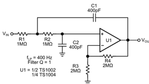
Figure 3: A Nanopower 2-Pole Sallen-Key Low-Pass Filter.
